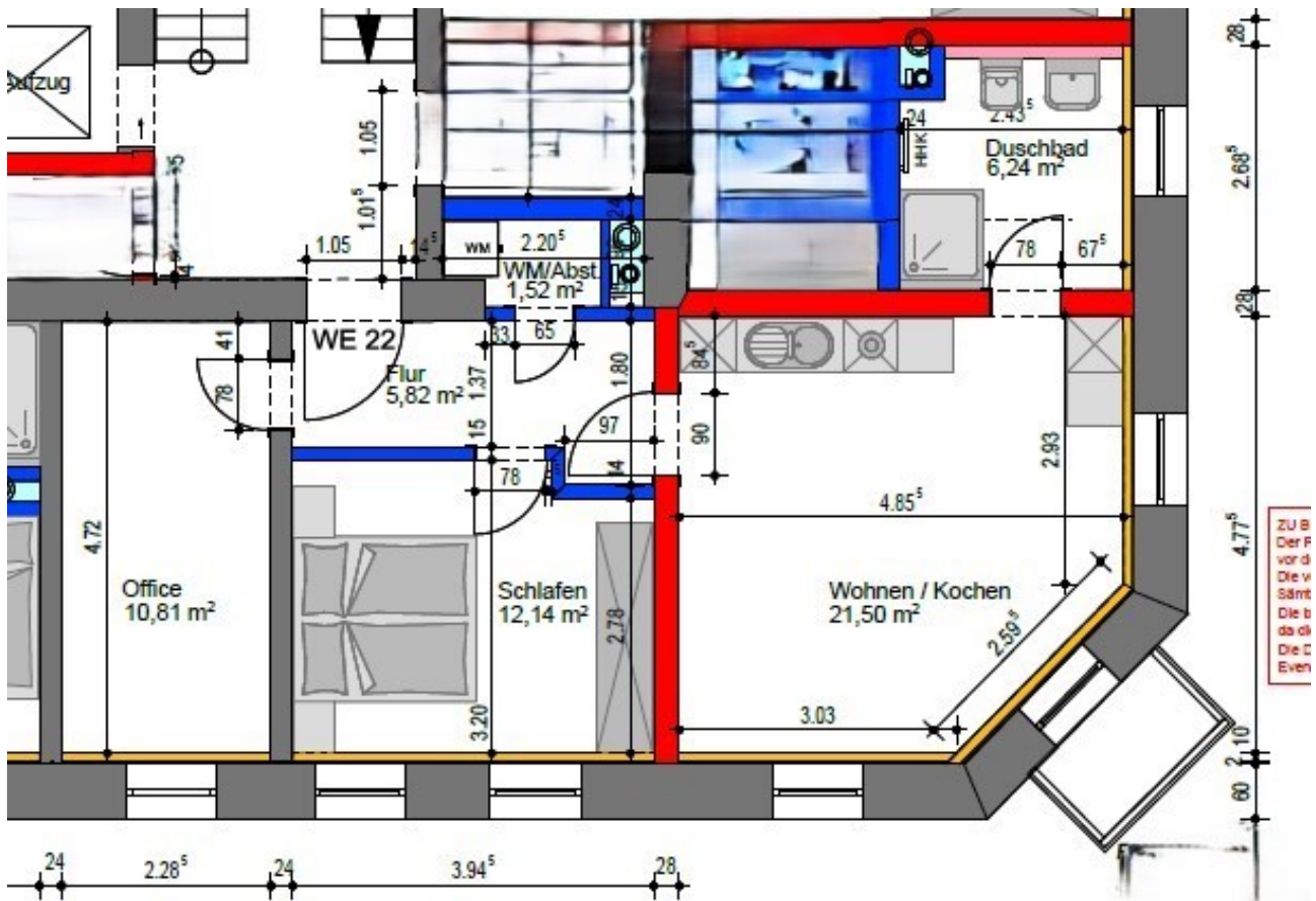
Grundriss WE 22
